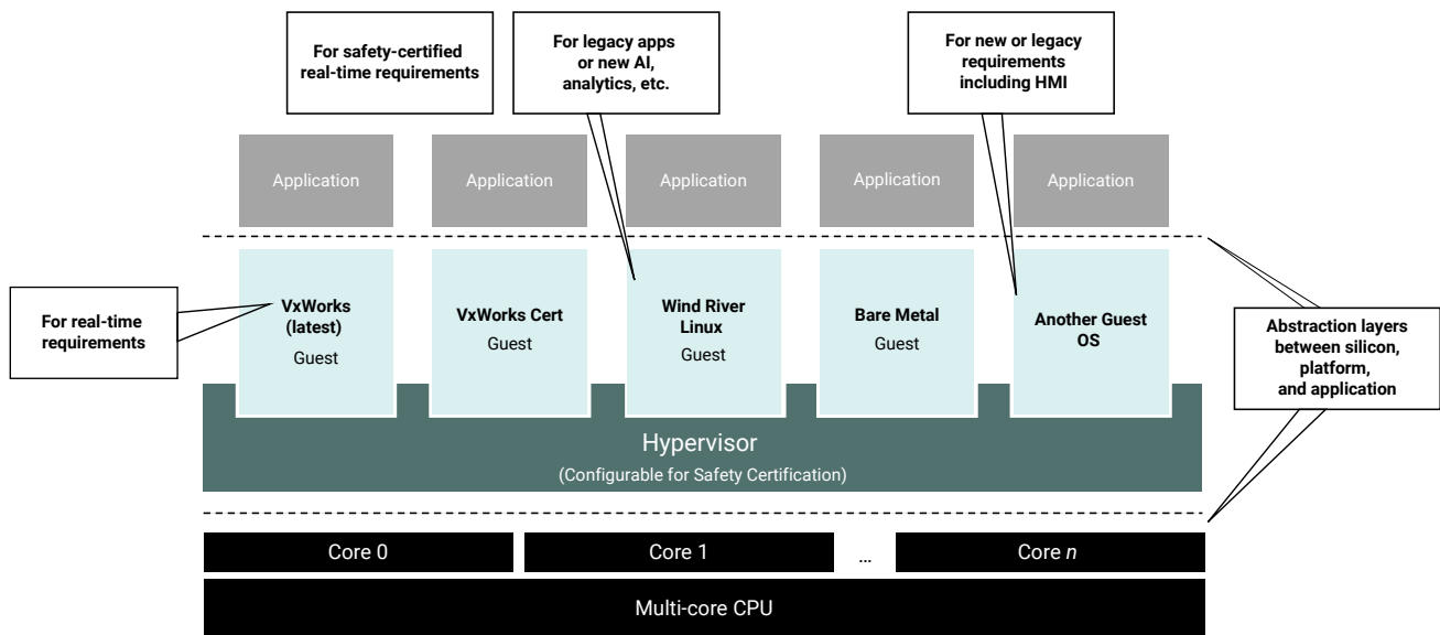
Figure 4. An example configuration of Wind River Helix Virtualization Platform
